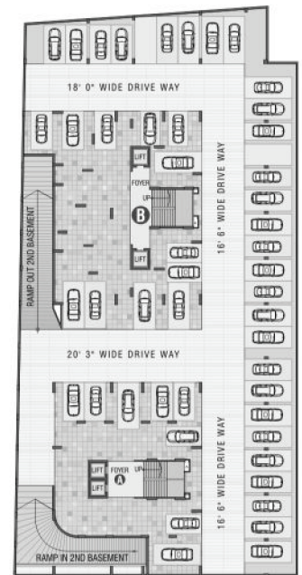
SECOND BASEMENT PLAN
